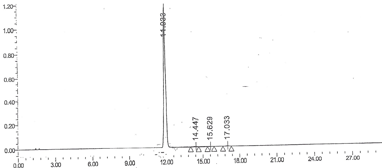
Auto-Scaled Chromatogram
